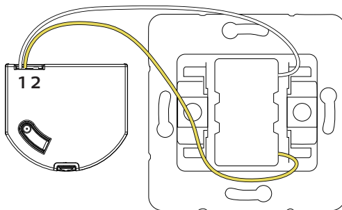
Standard switch with side mounting
