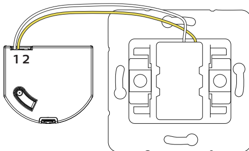
Standard switch with top mounted wires
